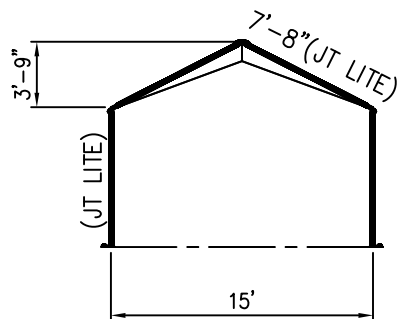
CENTER BAY
