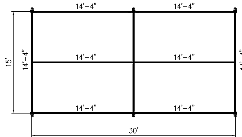
PLAN VIEW
