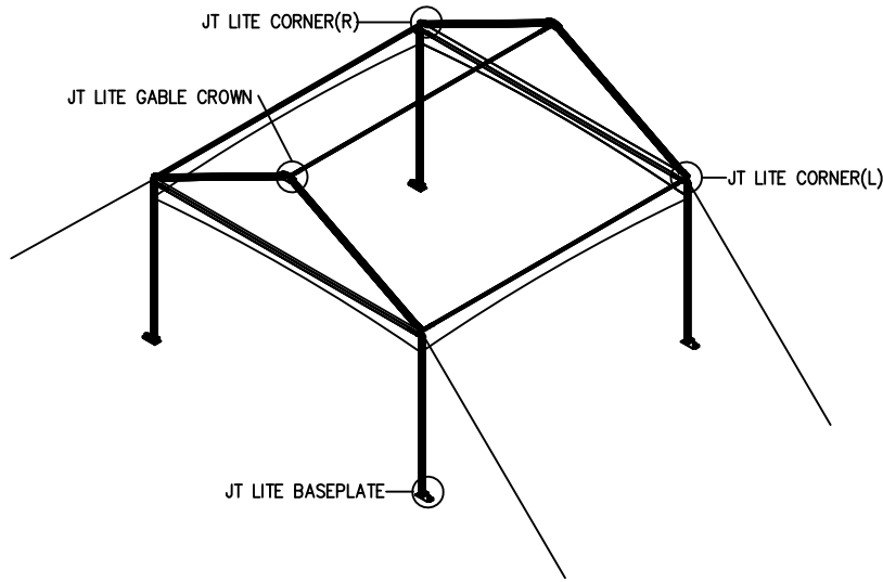
ISOMETRIC VIEW
