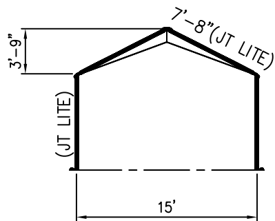
CENTER BAY
