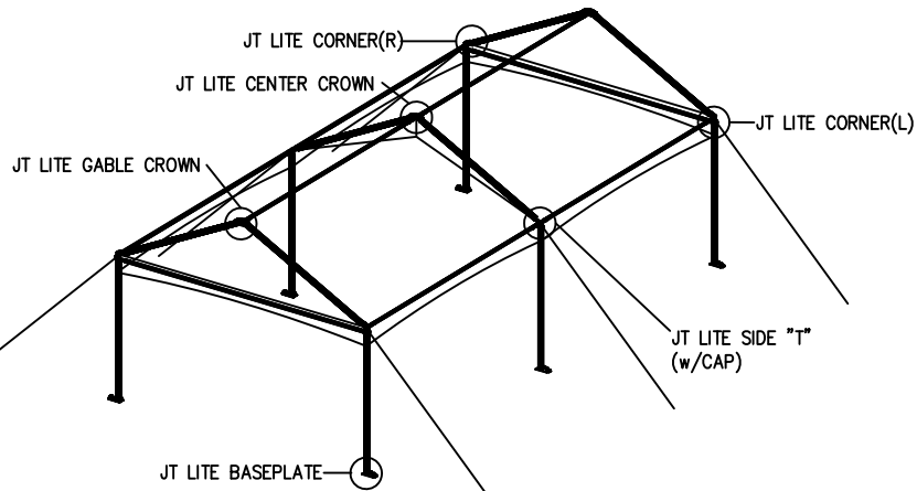
ISOMETRIC VIEW
